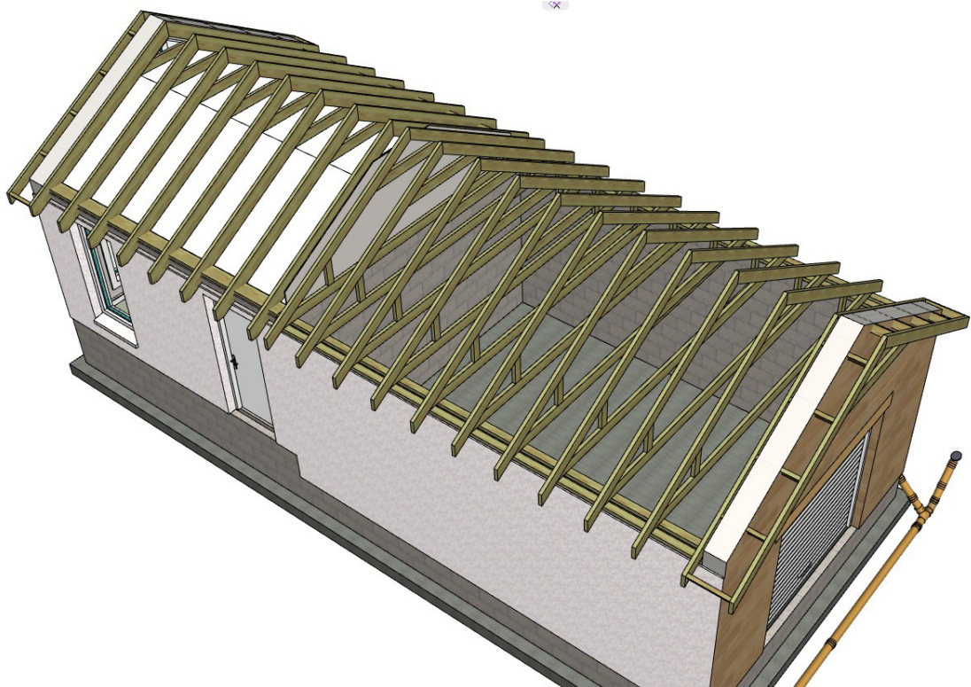
TRUSSES
